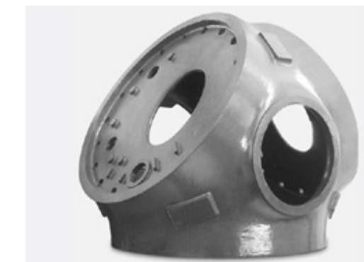
Rotor Hub
